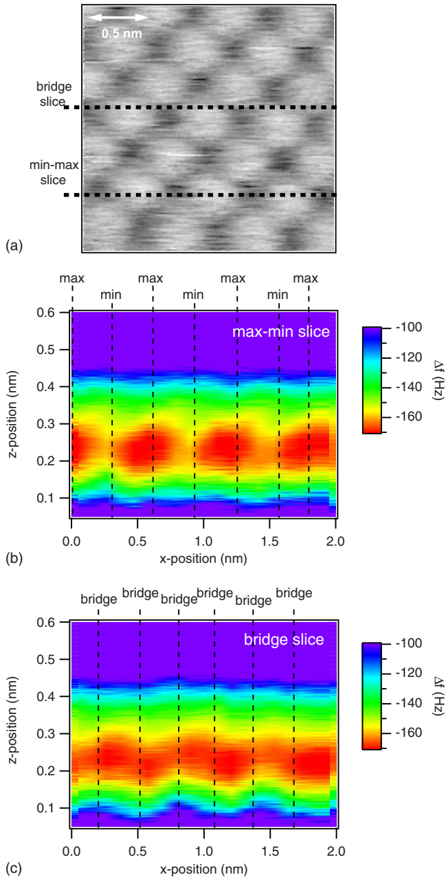
FIG. 1. (Color online) (a) Atomic resolution image obtained on the NaCl(001) surface at \Delta f = -144.9 Hz. (b) Slice of the three-dimensional frequency-shift data across the position of the topographic maximum and minimum. (c) Slice of the three-dimensional frequency-shift data across the bridge positions.
